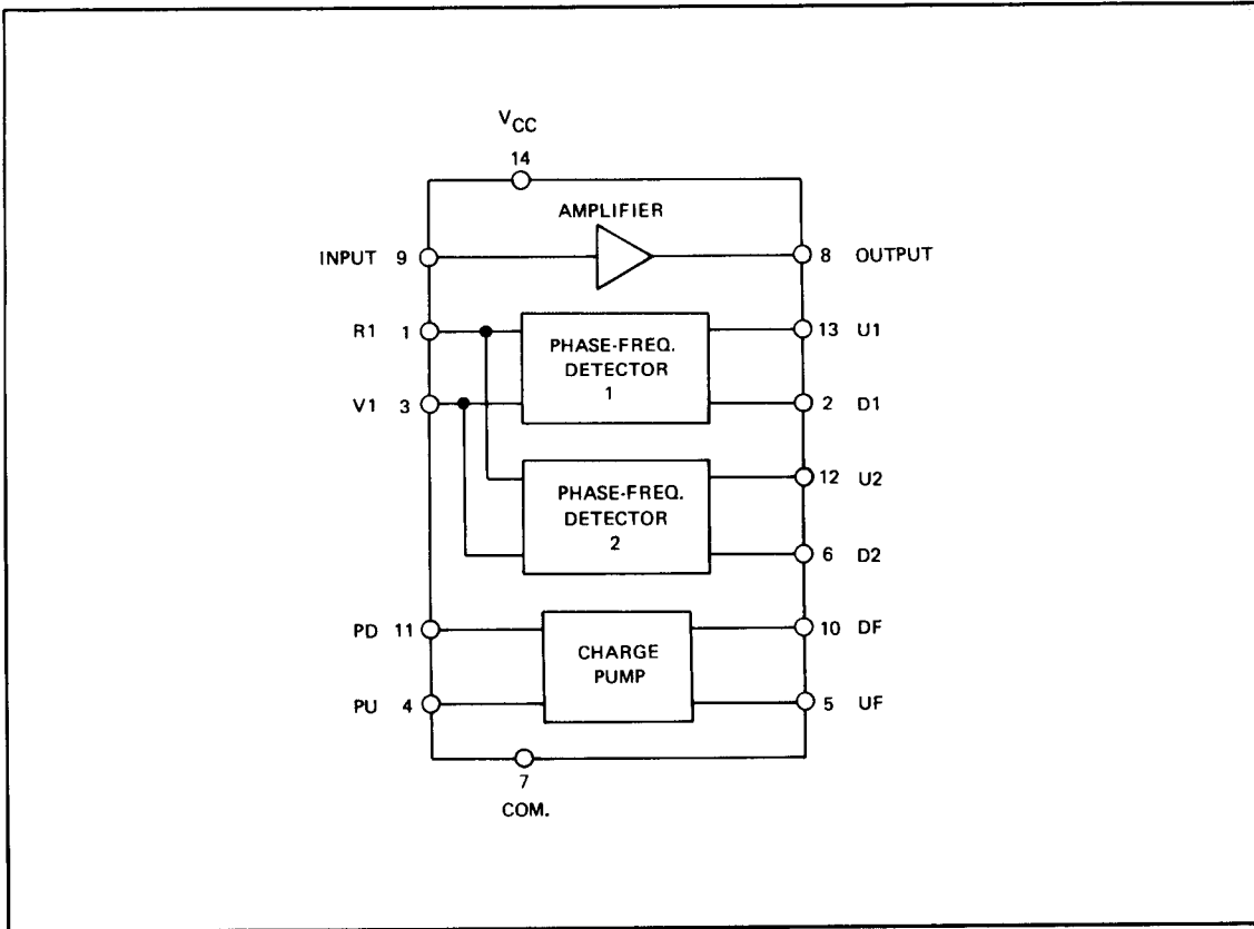
Figure 3-11. Phase-Frequency Detector
