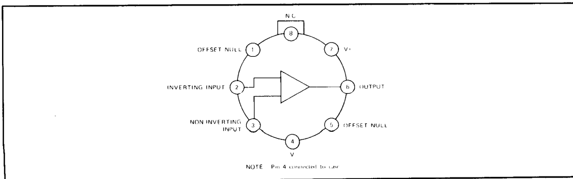
Figure 3-6. Operational Amplifier
